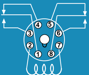
DPDT
