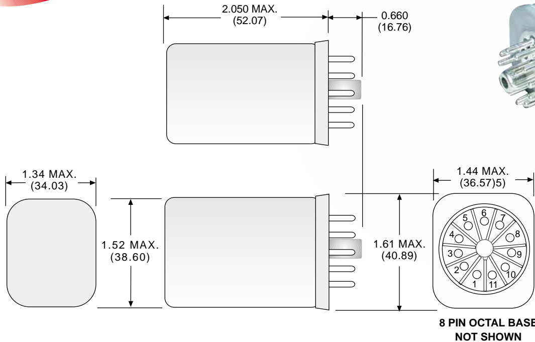
OUTLINE DIMENSIONS DIMENSIONS SHOWN IN INCHES & (MILLIMETERS).
